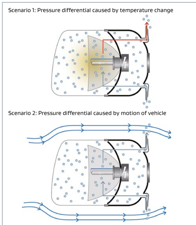
Figure 4: Temperature rise and vehicle motion lead to air circulation in headlamp
