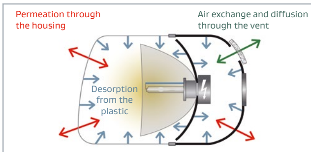
Figure 1: Three causes of moisture in vehicle headlamps
